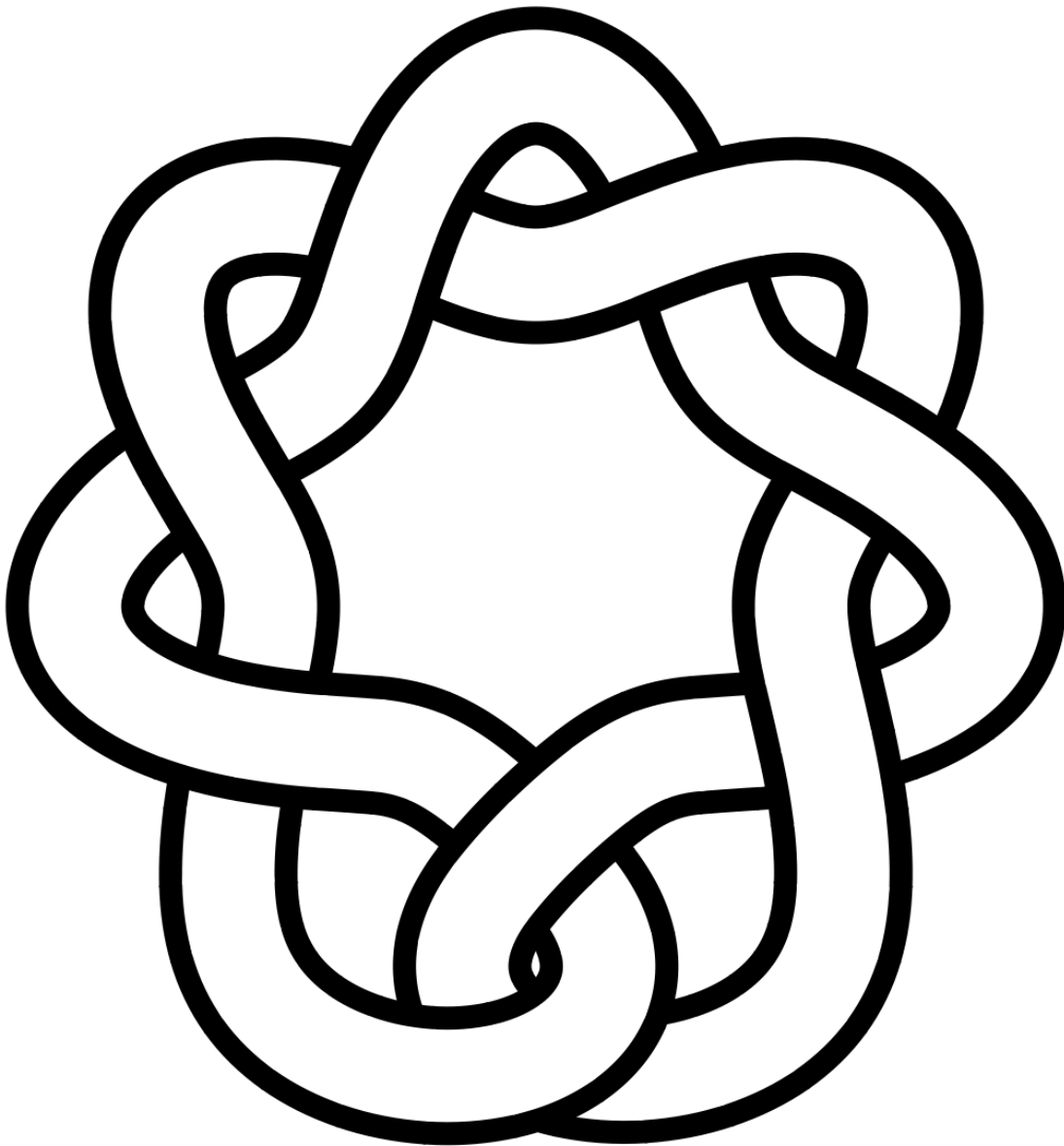
The \delta_1 Knot
